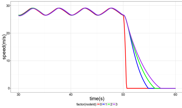
Figure 3: Naive Solution: Speed Changing
