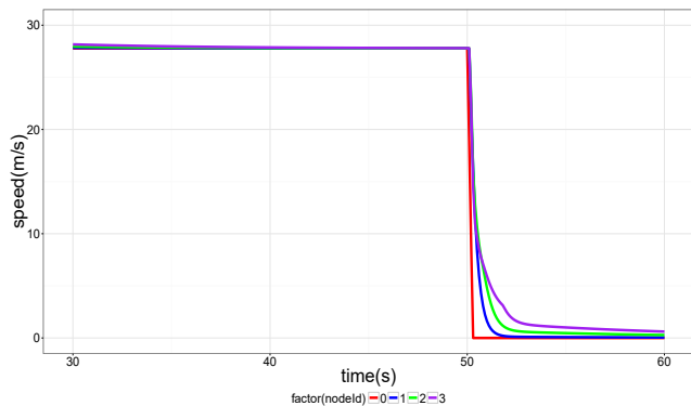
Figure 5: Speed Changes of Platoon : Distance
