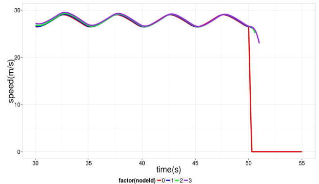
Figure 2: Speed Changes of Platoon during the Crash
