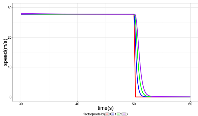
Figure 4: Speed Changes of Platoon : Acceleration
